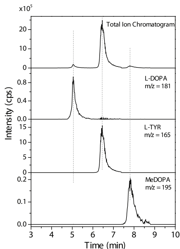
Figure 4. Total ion chromatogram and selected ion chromatograms for L-DOPA, L-tyrosine and \alpha -methyldopa of the GK Kormorán variety.
