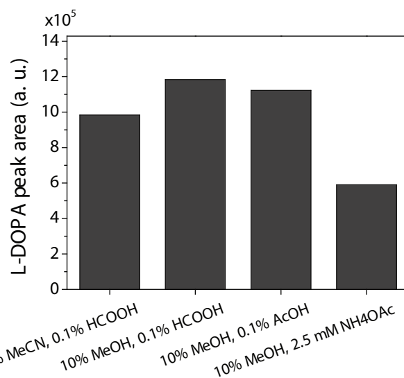
Figure 3. The effect of different mobile phase composition on the L-DOPA signal.
