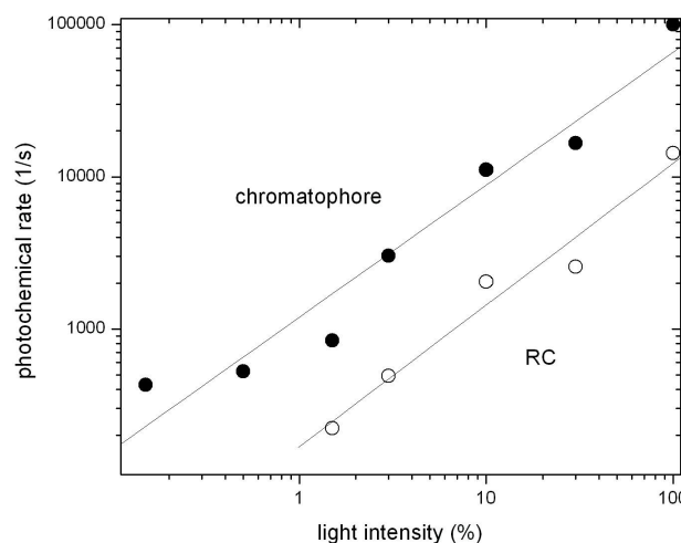
Figure 3. Comparison of the rates of the photochemical phase of the fluorescence induction excited by the same light intensities in chromatophores ( \bullet ) and isolated RCs ( \circ ). The light intensities were attenuated by calibrated neutral density filters. In double logarithm representation, the slopes are 0.87 (chromatophore) and 0.93 (RC) and the rate is 7 times higher in chromatophore than in isolated RC under identical light intensity.
